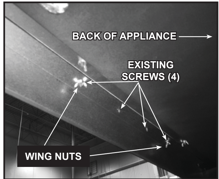
Figure 13. Secure Glass Baffle with Wing Nuts - Inside Top View
