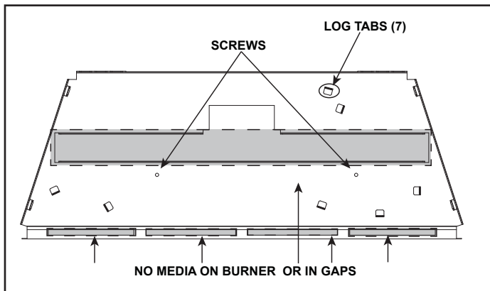
Figure 16. COSMO32-IFT Empty Base Pan
