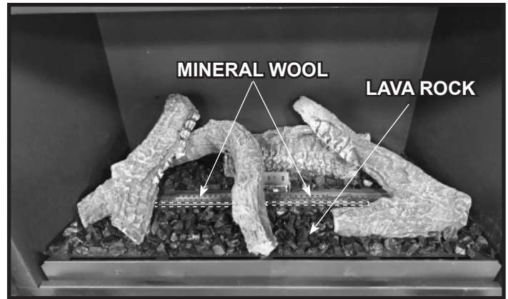
Figure 21. Properly Placed Lava Rock / Location for Mineral Wool
