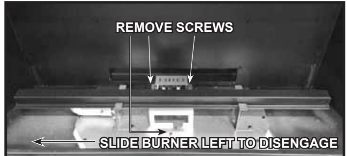
Figure 1. Remove Pilot Screws
