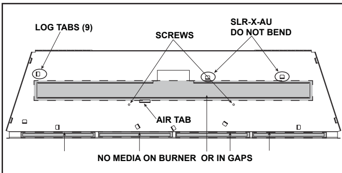
Figure 3. COSMO42-IFT Empty Base Pan
