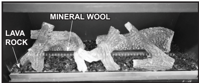
Figure 11. Properly Placed Lava Rock / Location for Mineral Wool
