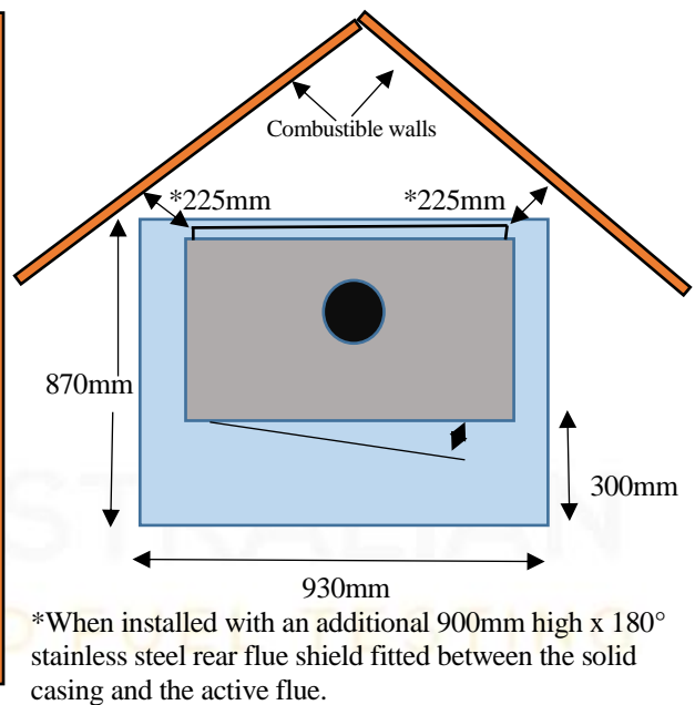
Figure 1 – Clearance Diagram
