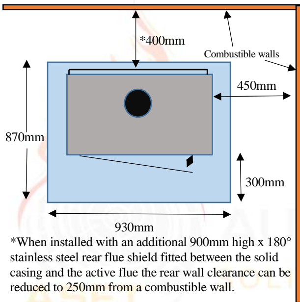
Figure 1 – Clearance Diagram
