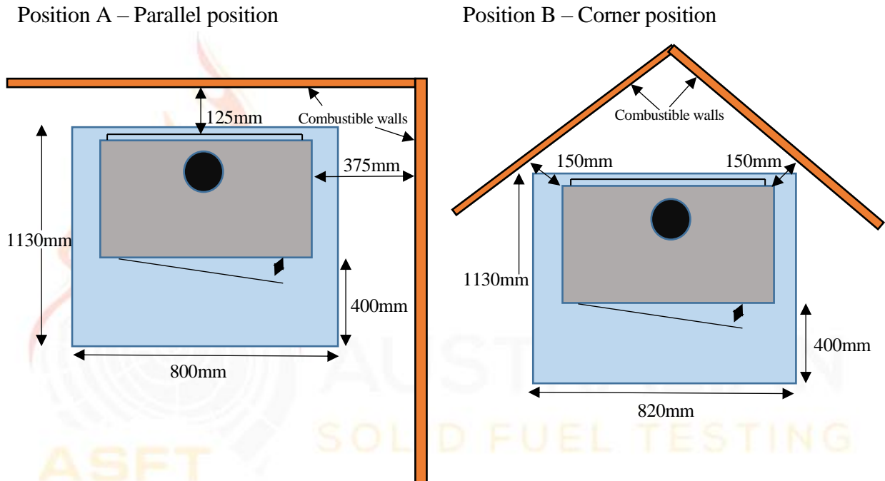
Figure 1 – Clearance Diagram
