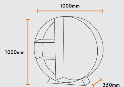
CIRCULAR STACKER H 1000mm | W 1000mm | D 350mm
