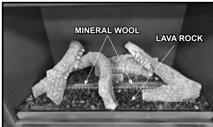
Figure 31. Properly Placed Lava Rock / Location for Mineral Wool
