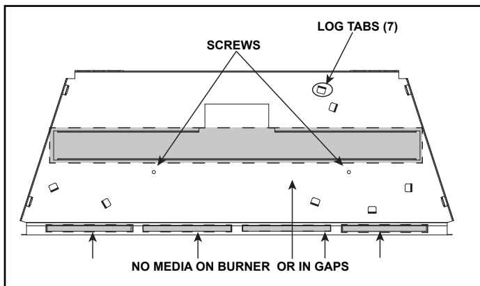
Figure 26. COSMO32-IFT/COSMO32-IFT-B Empty Base Pan
