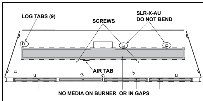
Figure 3. COSMO42-IFT/COSMO42-IFT-B Empty Base Pan
